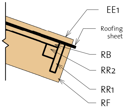
3) Roof Reinforcement
